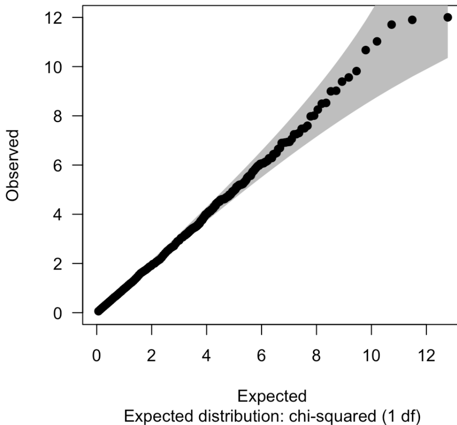
QQ plot
